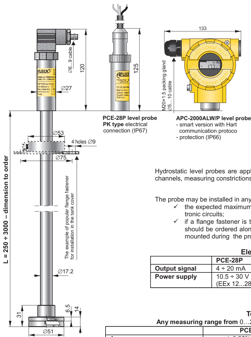
PCE-28P level probe PD type electrical connection (DIN 43650) (IP65)
