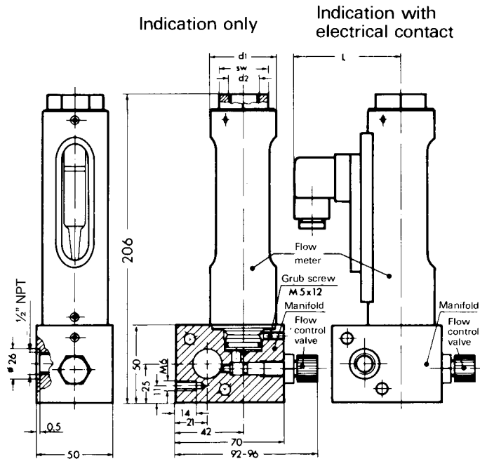
Diagram 2: Dimensions
